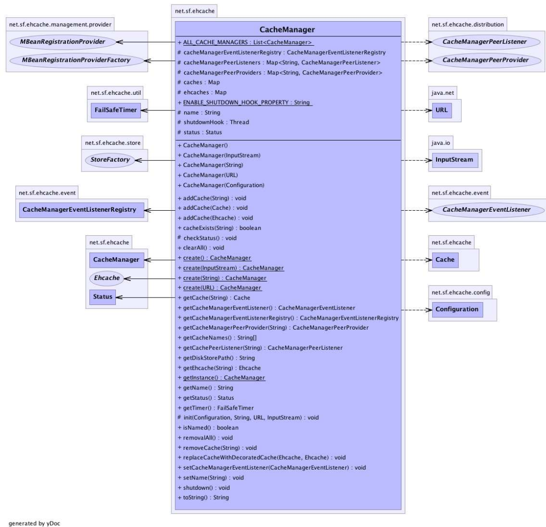
CacheManager Class Diagram
